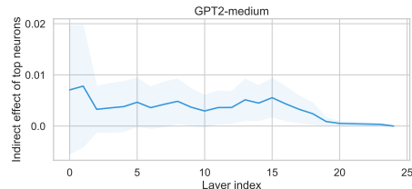
Figure 8: Indirect effects of top neurons in GPT2-medium for gender-neutral interventions on the professions dataset. Here, the effect is distributed across all layers.
