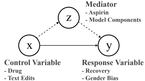
Figure 1: Mediation analysis illustration.
